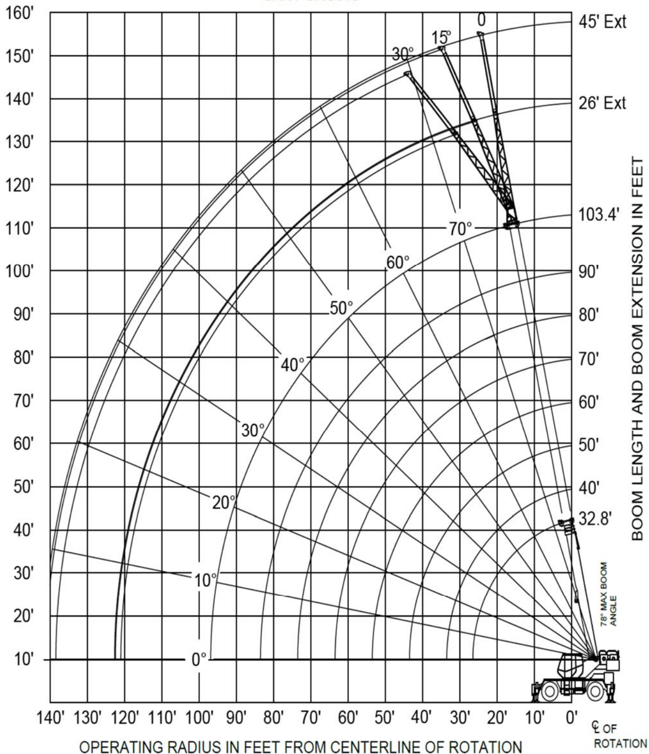
WORKING RANGE DIAGRAM (BOOM DEFLECTION NOT SHOWN) SANY SRC840
